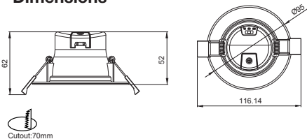
DL1195-WHTC7S01
