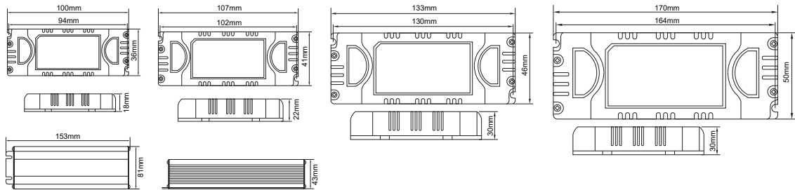
3A-DR-CV-20/30/60/80/100/150/200-24 with AU Plug
