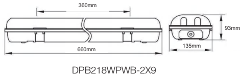
DPB218WPWB-2X9
