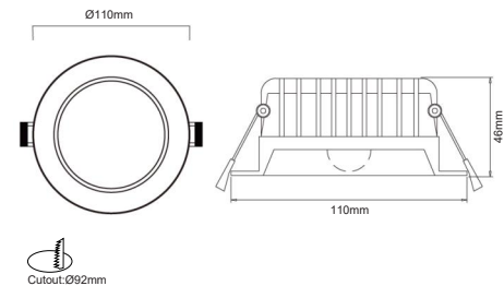
AL5007-WHTC10S02-TS
