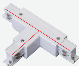
T Connector-R1-4 wires
