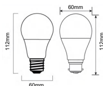
LED-A60-11W
