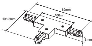
T-Feed-R2-3 wires
