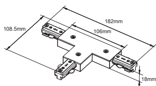
T-Feed-L1-3 wires
