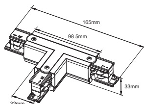
T Connector-L2-4 wires
