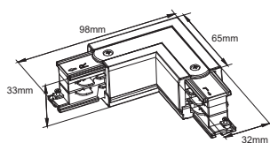
“L” Right Container-4 wires
